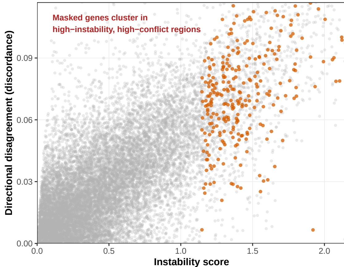
Instability captures subgroup conflict
