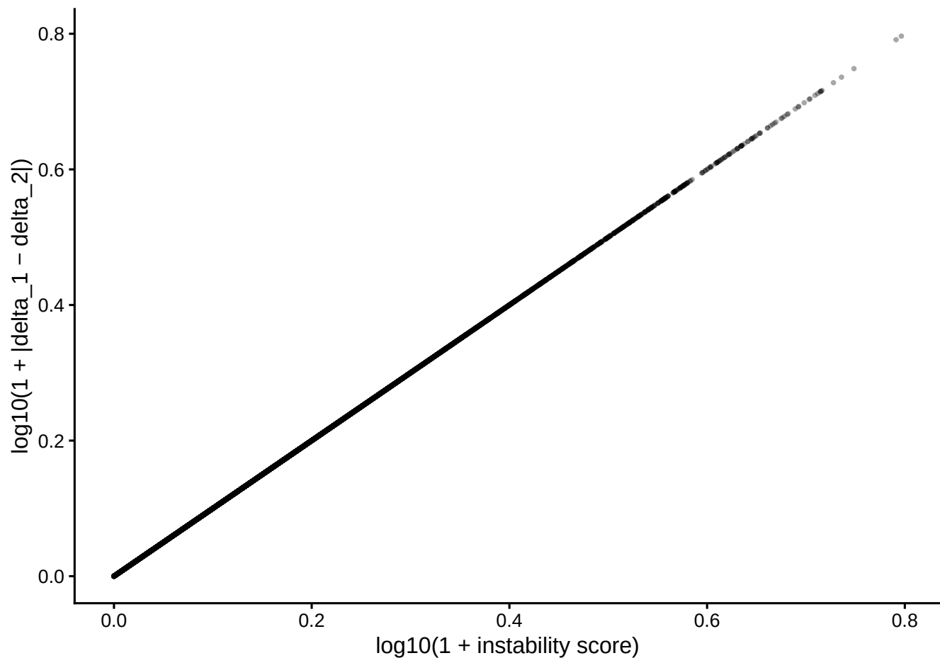
DES: Instability vs subgroup effect divergence
