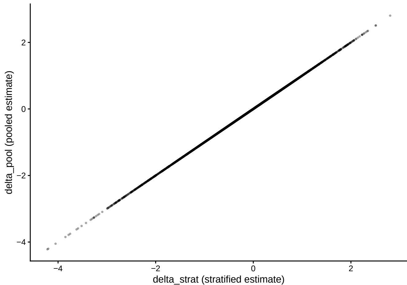
DES: Pooled vs stratified effect estimates
