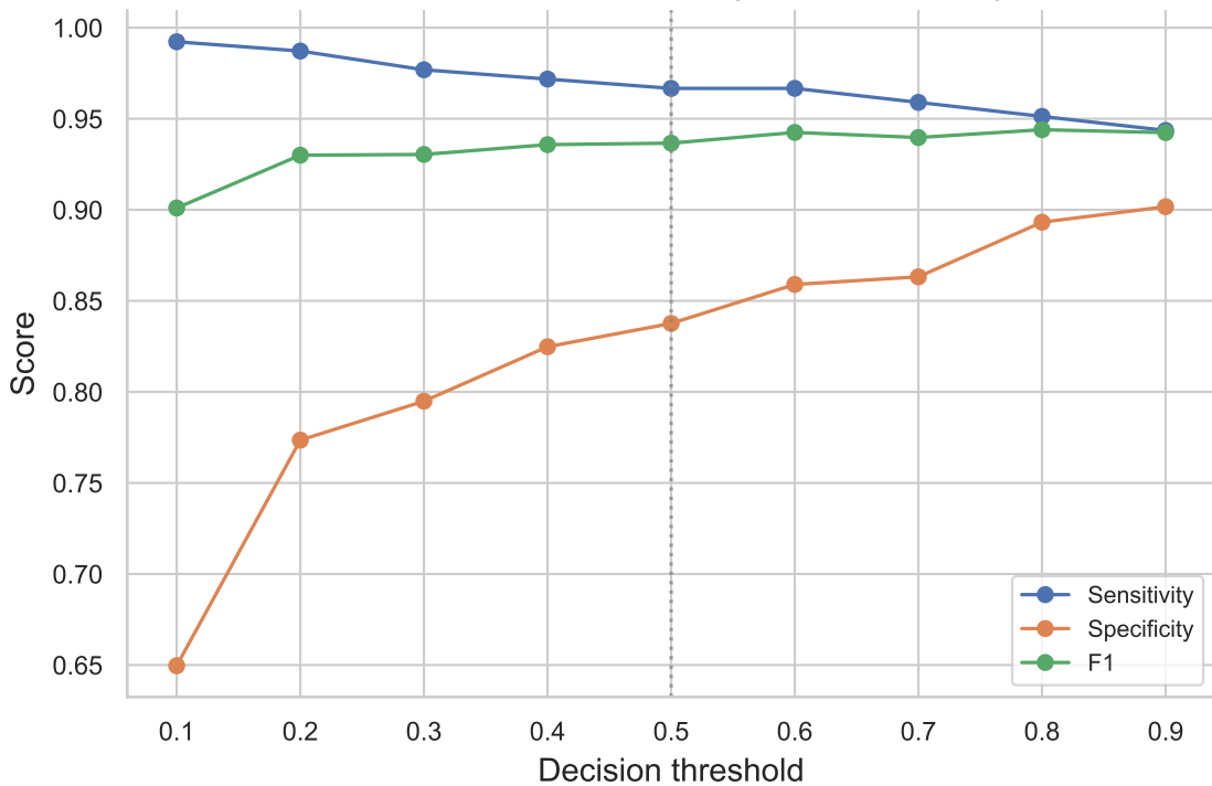
Threshold Robustness (EfficientNet-B0)
