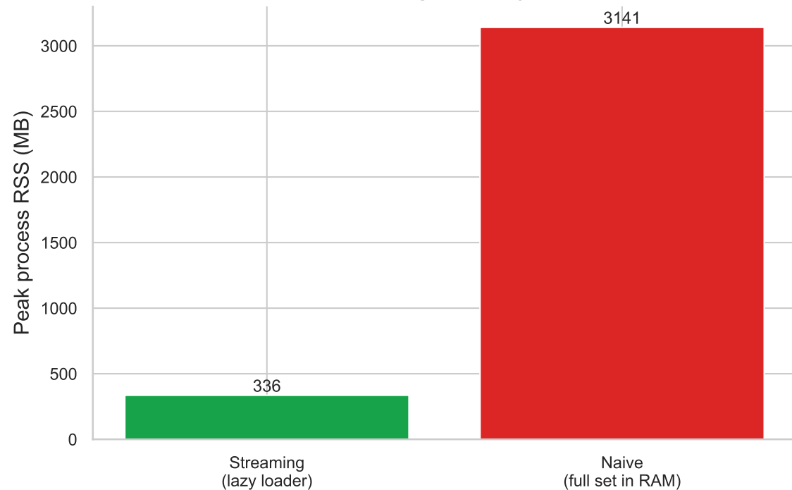
Dataset Loading: Memory Footprint
