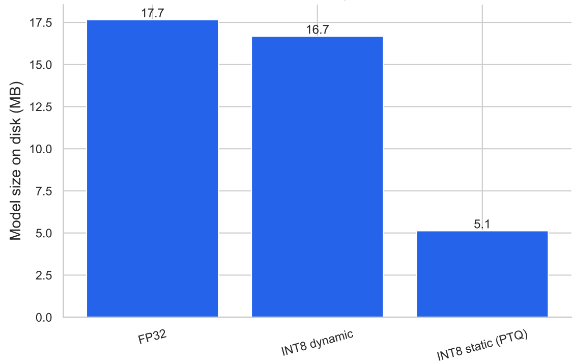
Model Footprint by Precision
