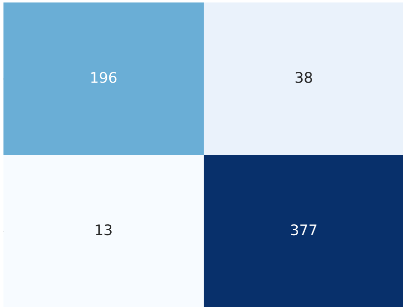
Confusion Matrix
