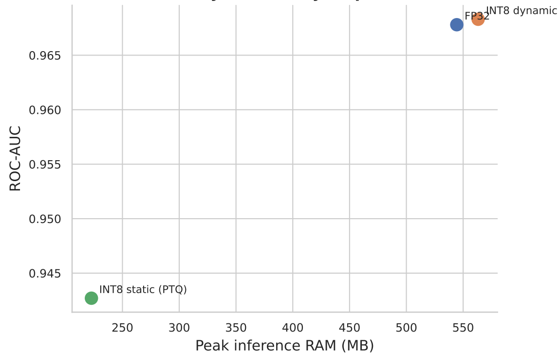
(B) Accuracy vs memory — quantization
