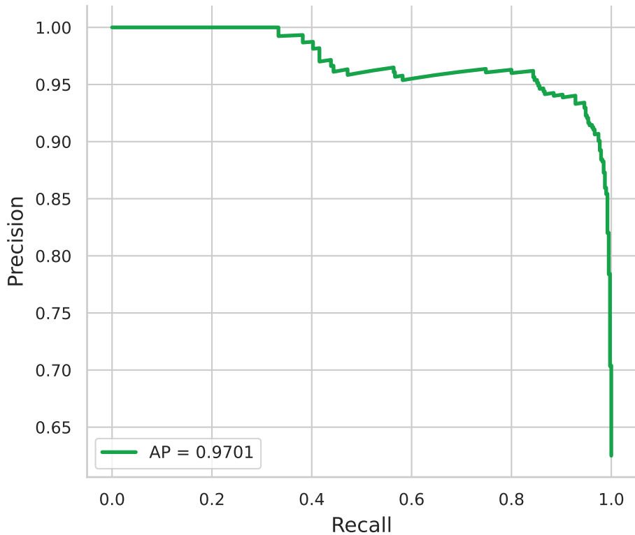
Precision-Recall Curve
