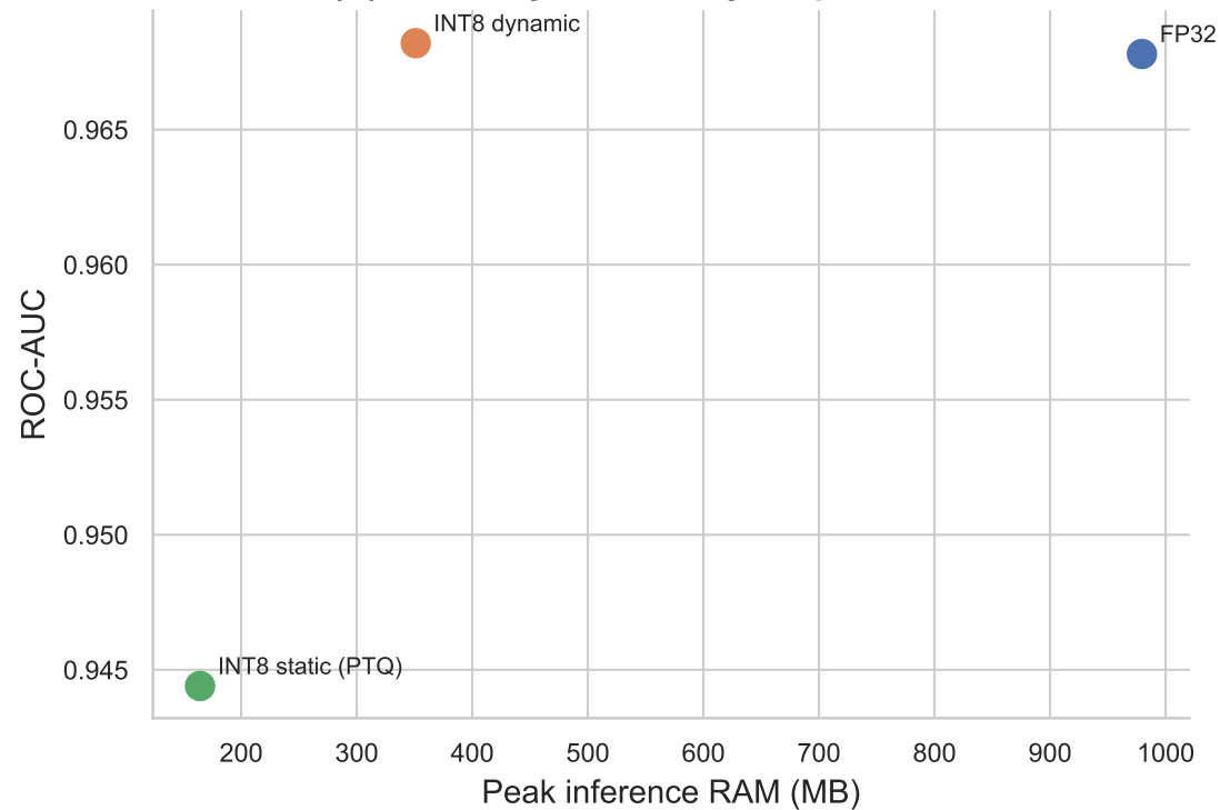
(B) Accuracy vs memory — quantization
