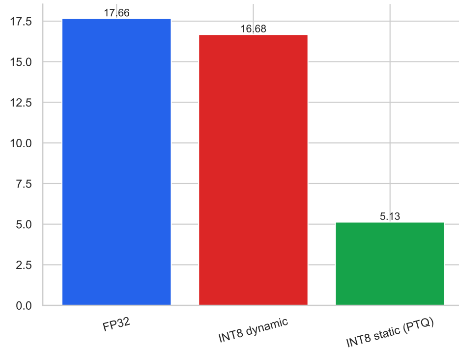
Model Size (MB)
