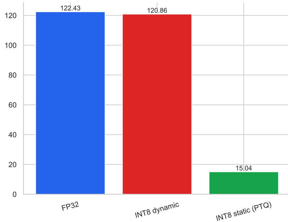
Latency (ms/img)
