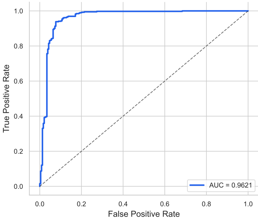
ROC Curve
