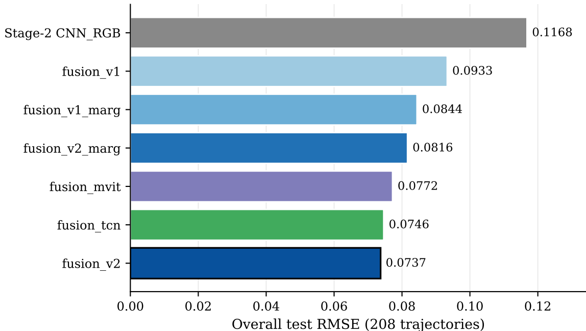
Overall RMSE — all models on the matched 208-trajectory test set
