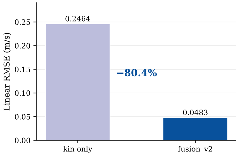
Linear — kin alone vs fusion
