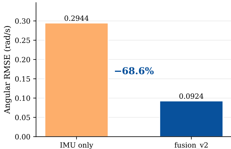
Angular — IMU alone vs fusion
