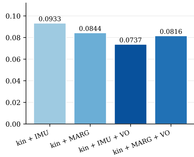
Overall RMSE
