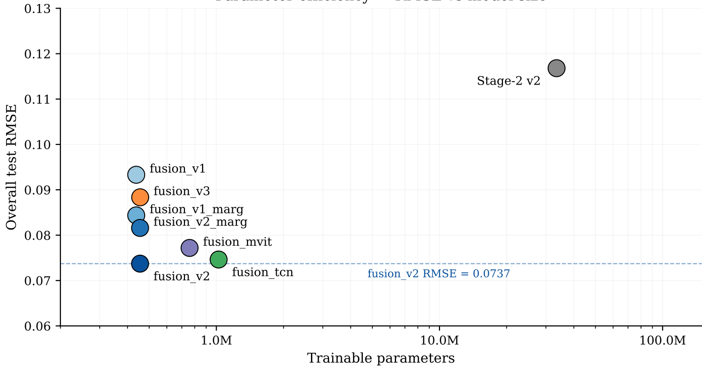
Parameter efficiency — RMSE vs model size
