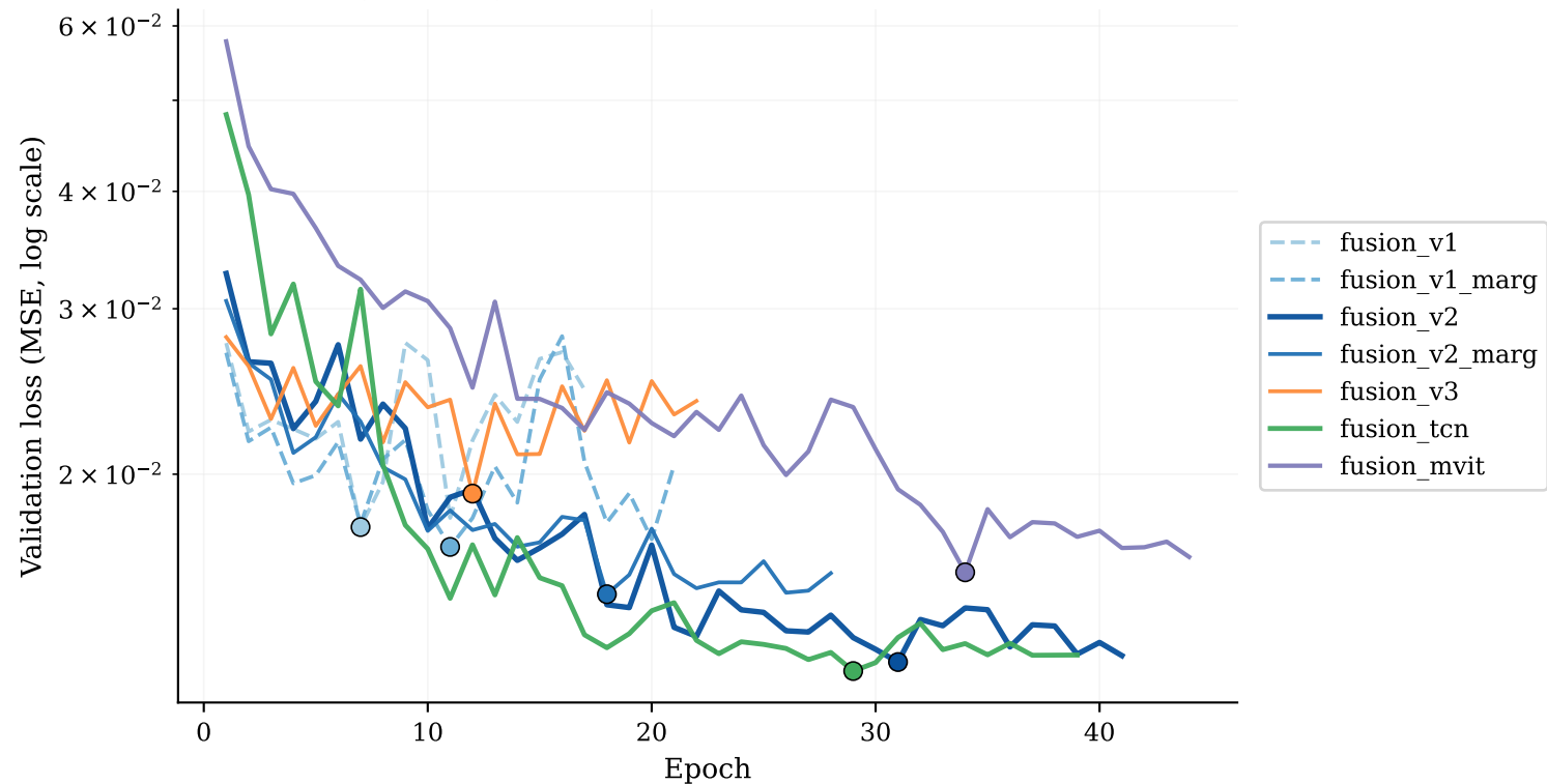
Validation loss during training — all fusion variants (• = best epoch, dashed = no VO)
