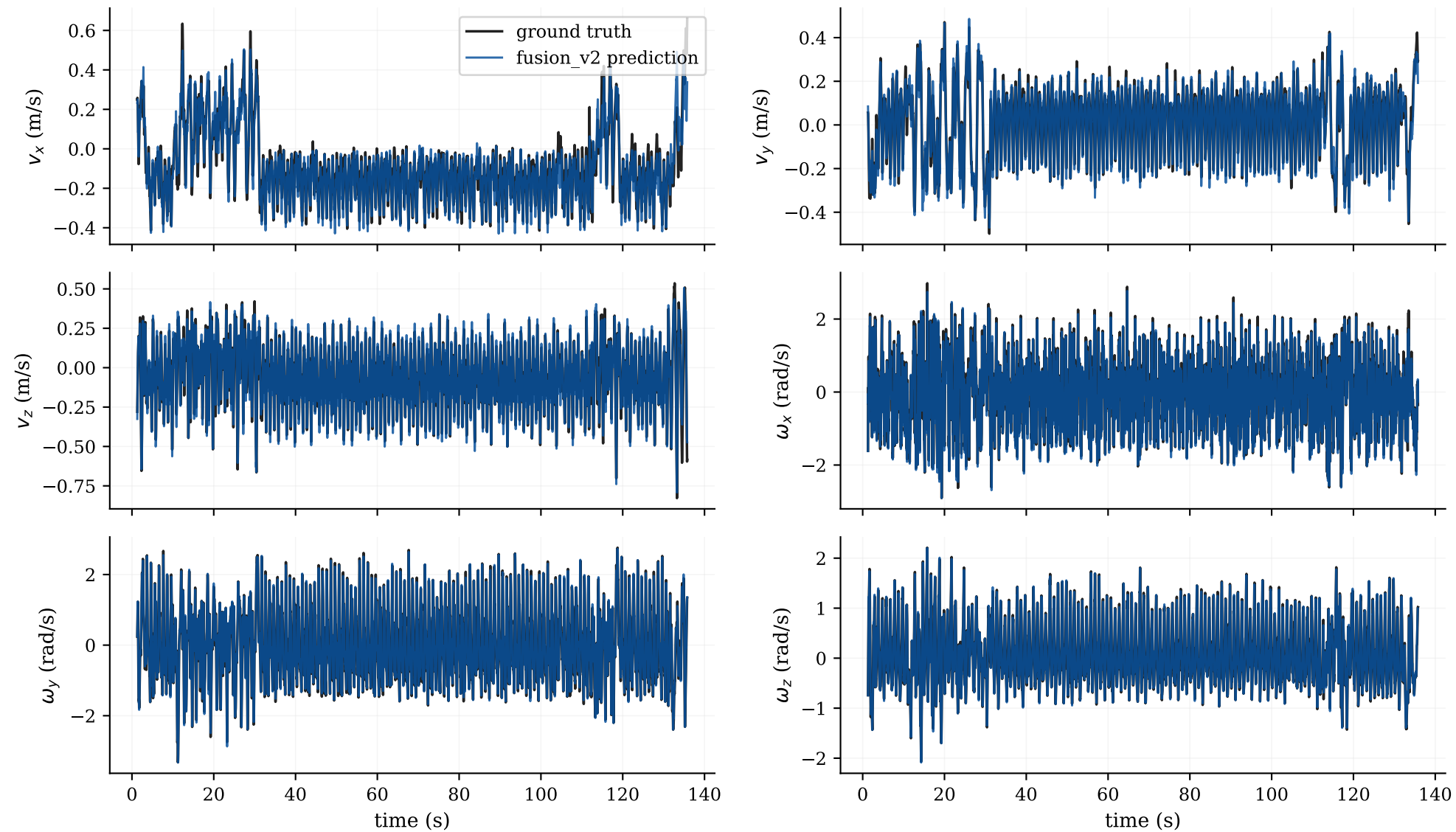
Sample test trajectory — fusion_v2 prediction vs ground truth (trajectory_000803_20260325_214110, ~median per-trajectory RMSE)
