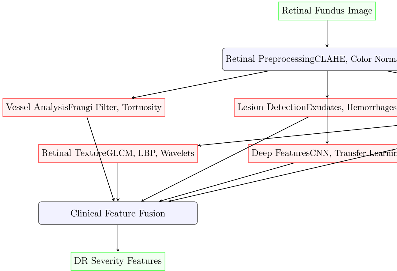
Figure 3: Specialized Architecture for Diabetic Retinopathy Feature Extraction
