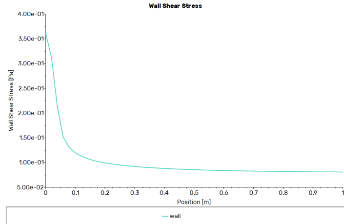
Figure 4: Variation of wall shear stress along the pipe length.
