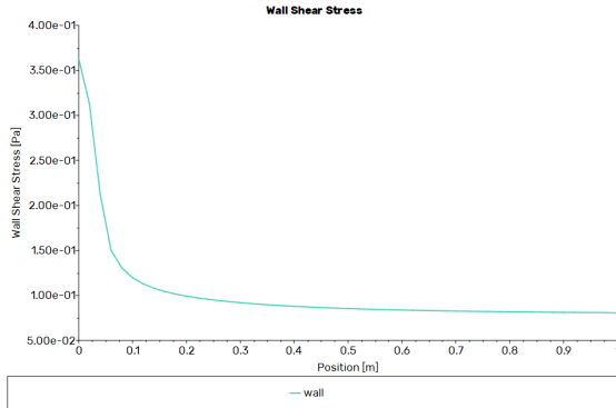
Variation of wall shear stress along the pipe length.
