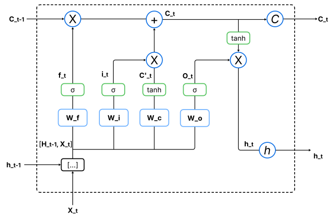
FIGURE 3. The internal structure of a single LSTM cell
