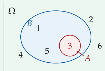
Restricting Sample Space to B
