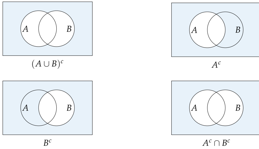
Figure 3: Fig: Visualization of De Morgan's Law (A \cup B)^c = A^c \cap B^c
