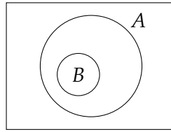
Figure 1: Visualization of proper and improper subsets
