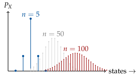
(b) Varying n ( p = 0.5 ). For large n , it can be approx. by Gaussian. Variance only increases. Density of states increases.
