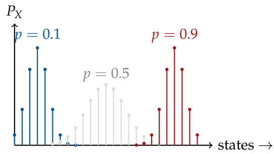
(a) Varying p ( n = 60 ). The PMF shifts right because E[X] = np . Variance increases then decreases (see graph p(1-p) ).
