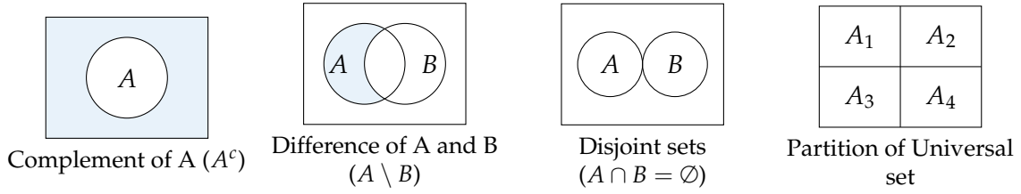
Figure 2: Visualization of complement of A, difference of A and B, disjoint sets and partition of universal set
