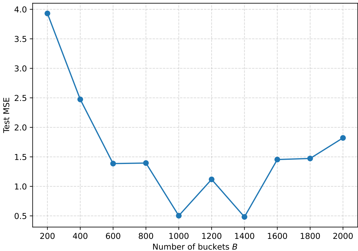
Expander-L: sensitivity to B
