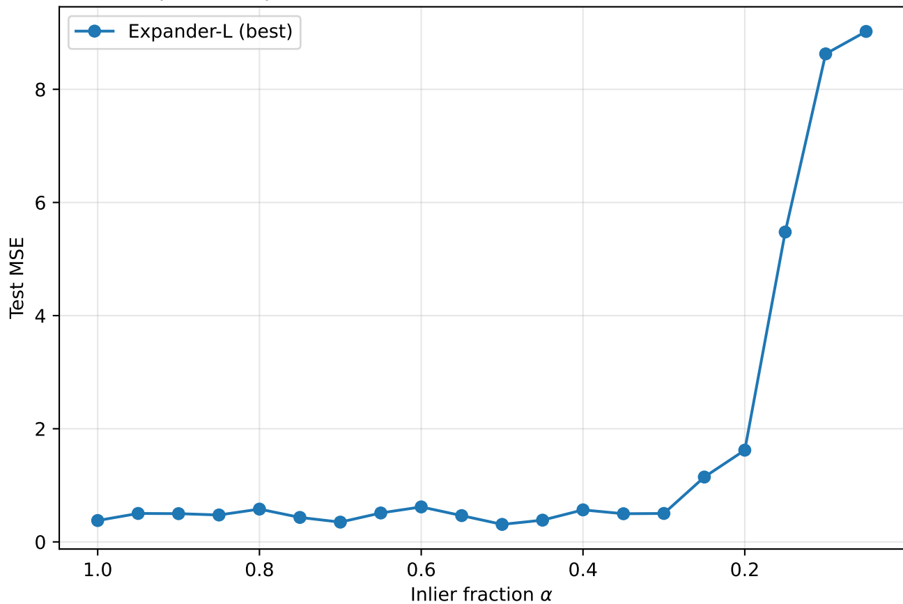
Expander-L performance vs \alpha (mode=uniform, n=5000, d=20)
