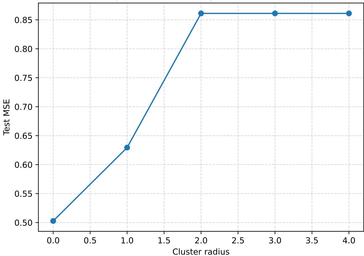
Expander-L: sensitivity to cluster radius
