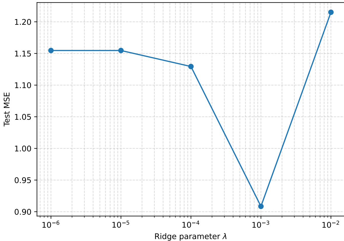
Expander-L: sensitivity to \lambda
