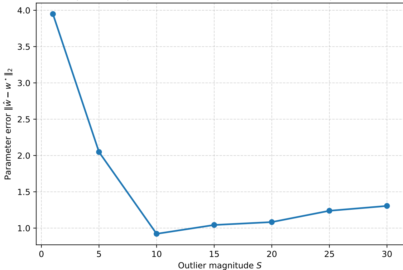
Expander-L: parameter error vs outlier magnitude ( \alpha=0.3 )
