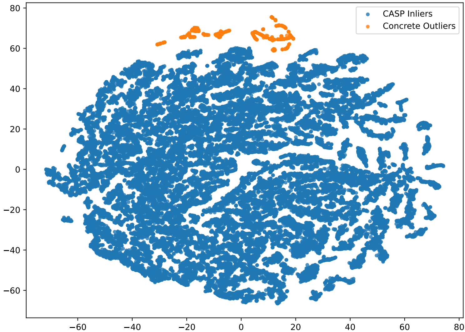
t-SNE of CASP (inliers) + Concrete (outliers)
