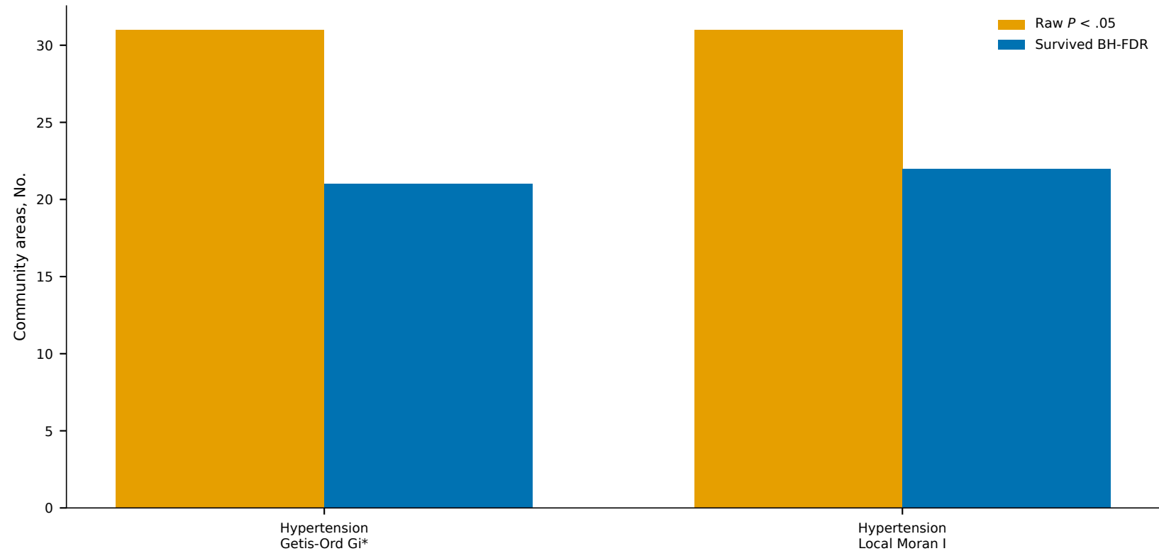
eFigure 12. Spatial classification survival after FDR control Community-area local signals before and after FDR control
