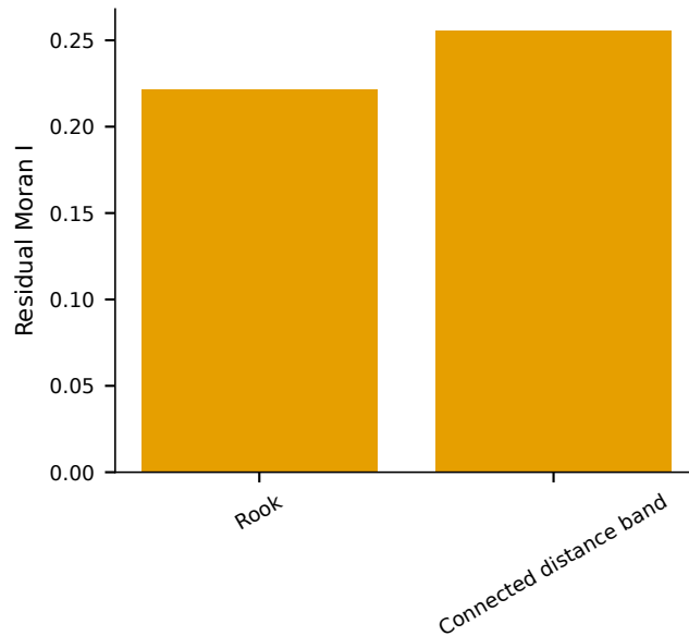
eFigure 10. COPD residual spatial dependence and sensitivity
