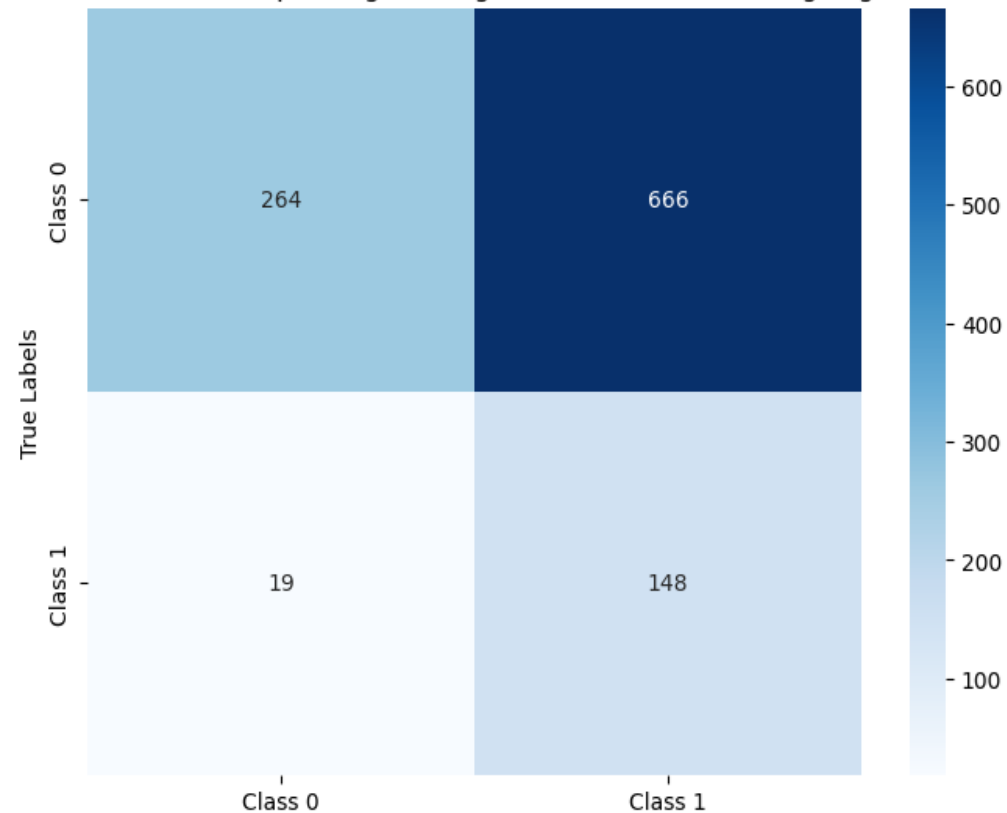
Confusion Matrix Heatmap of Logistic Regression with Class reweighing (Test set)
