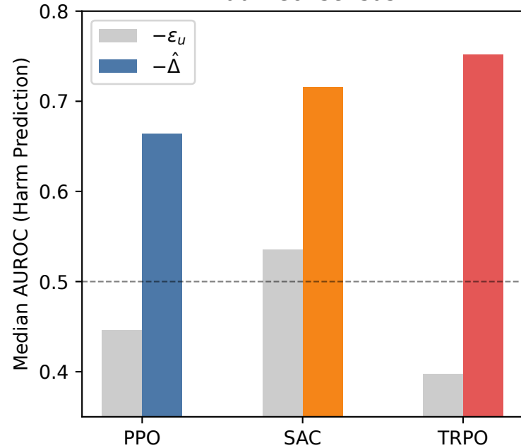
Audit Consensus
