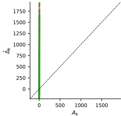
HalfCheetah
