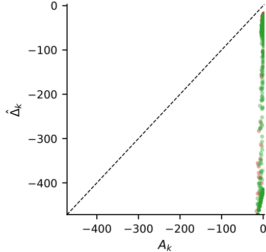
Acrobot
