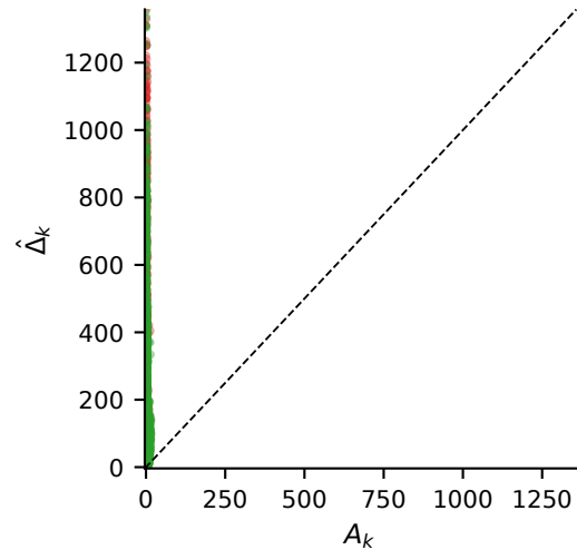
Hopper
