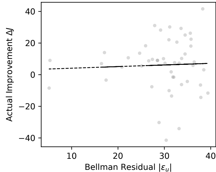
Absolute Residuals: Blind
