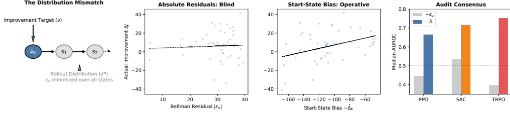
Figure 1: Headline result. (Left) Absolute Bellman residual |\epsilon_u| vs. ground-truth improvement \Delta J_k on Humanoid-v5 (a representative env): the cloud is flat. (Center) Start-state bias -\hat{\Delta}_k vs. \Delta J_k on the same updates: a clear linear relationship. (Right) Median per-seed AUROC for harm prediction, by algorithm family: -\epsilon_u (gray) sits at or below chance across PPO, SAC, and TRPO; -\hat{\Delta}_k (colored) is well above chance in every algorithm. The full per-environment table is Table 1.
