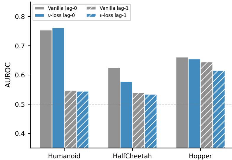
Harm-prediction AUROC
