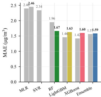
(c) Mean absolute error
