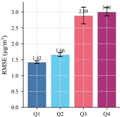
(a) Prediction RMSE
