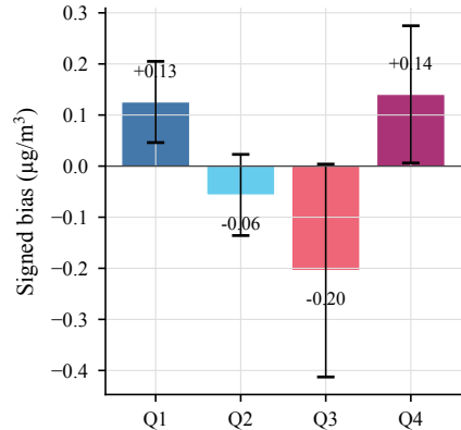
(c) Directional bias (pred – obs)
