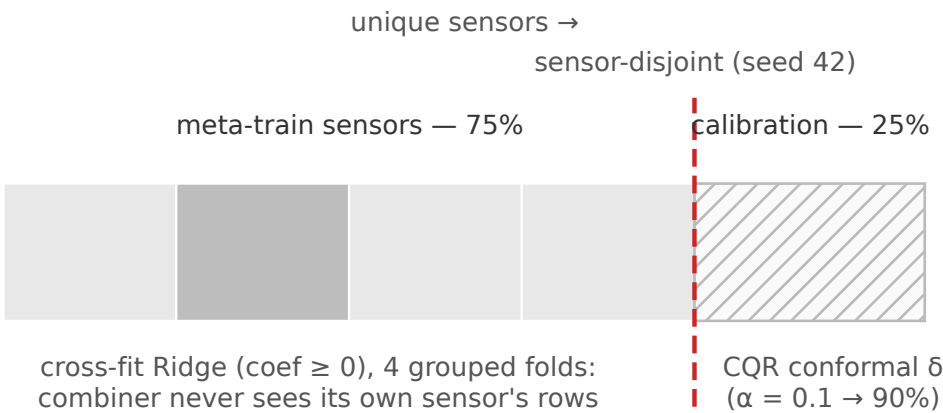
(e) Tier-3 meta split — cross-fit vs calibration
