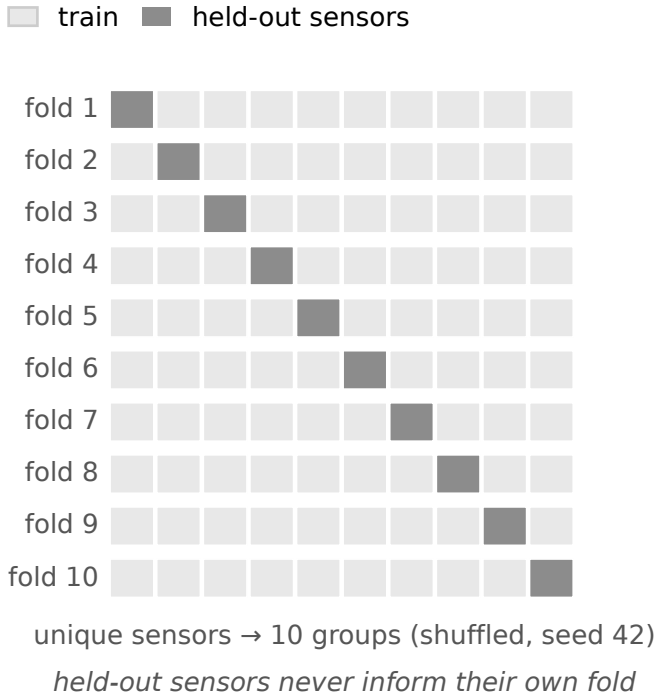
(a) LOSO — GroupKFold(10) over sensors
