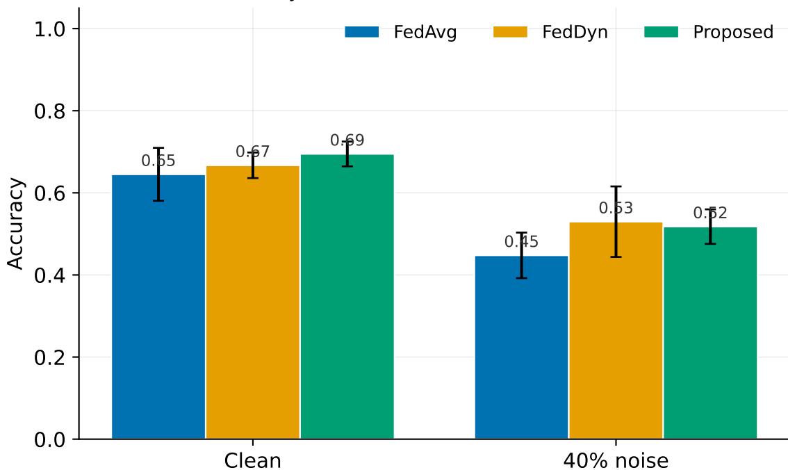
Accuracy — OCTMNIST (3 seeds, mean \pm std)
