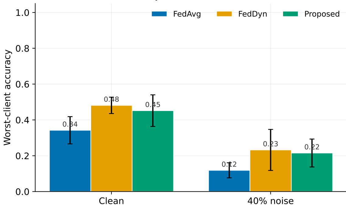
Worst-client accuracy — OCTMNIST (3 seeds, mean \pm std)
