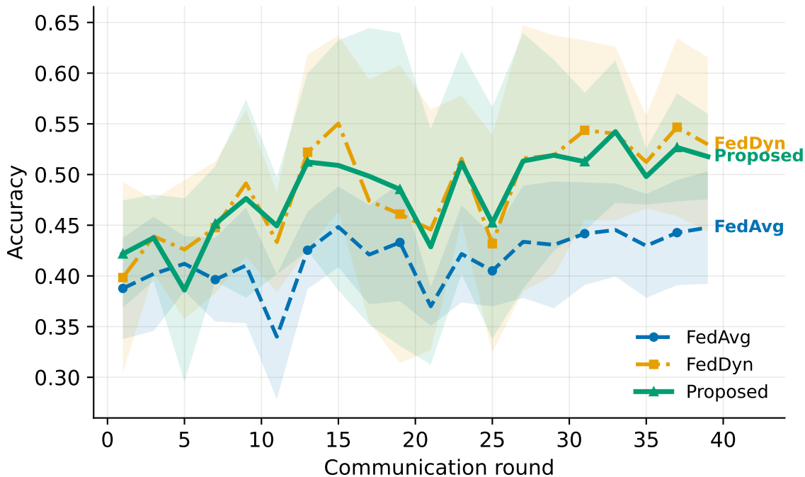
Accuracy over training — 40% label noise
