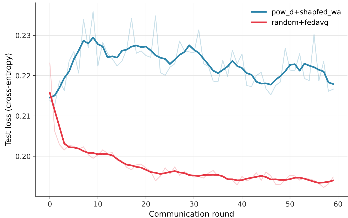
Test loss over rounds
