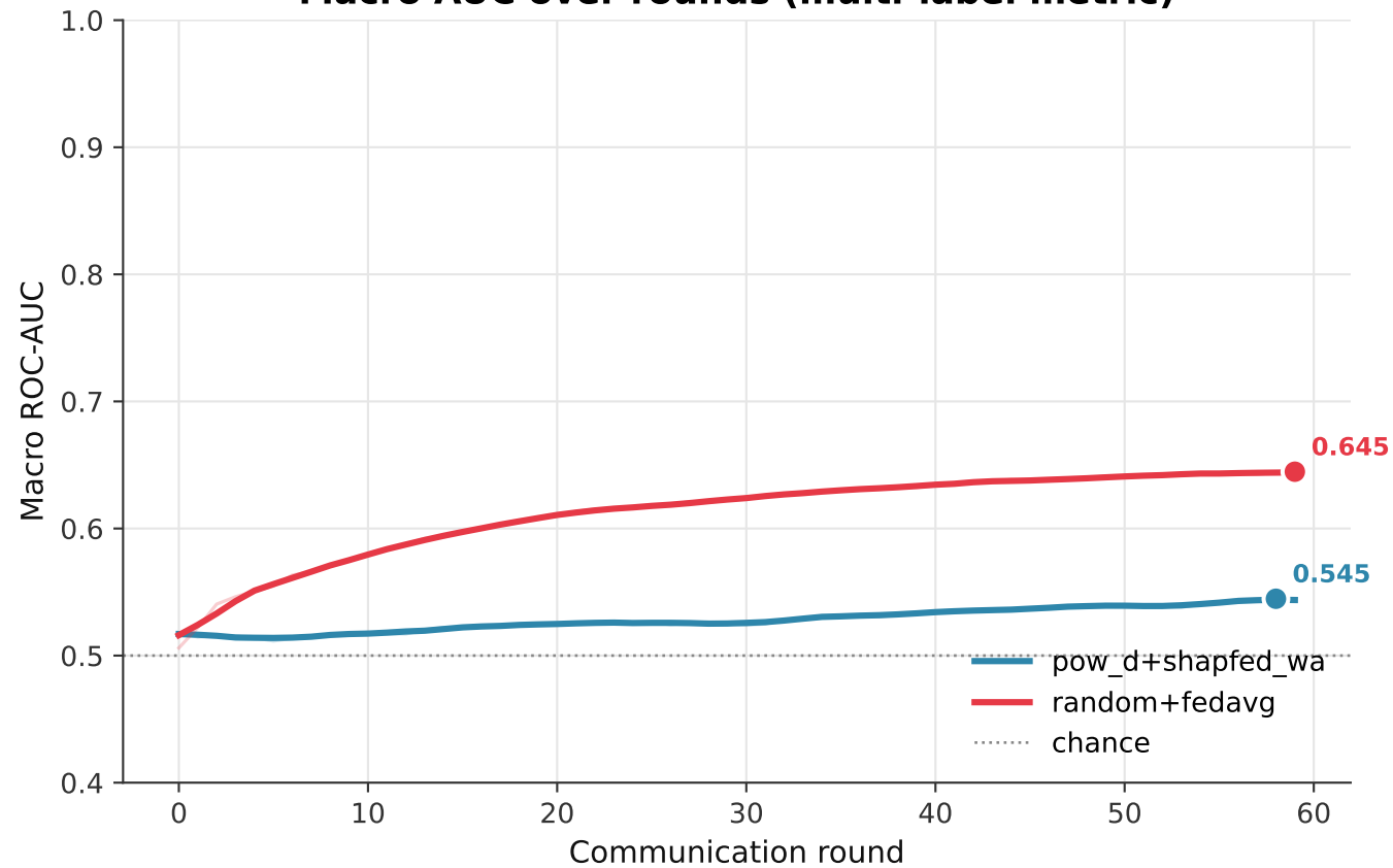
Macro AUC over rounds (multi-label metric)
