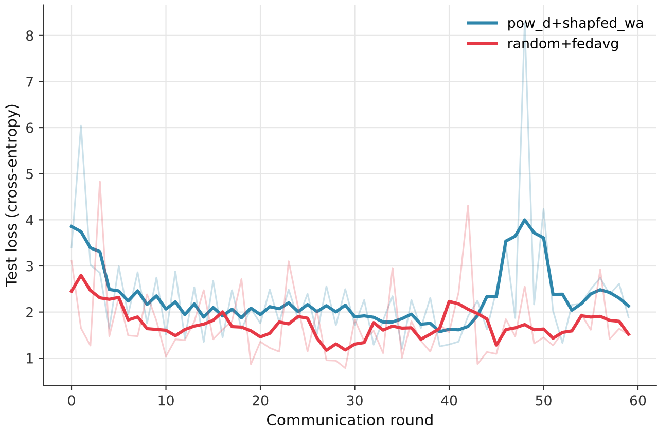
Test loss over rounds
