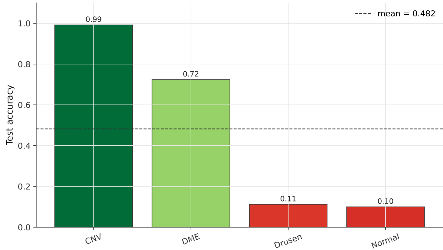
Per-class accuracy at round 59 — random+fedavg
