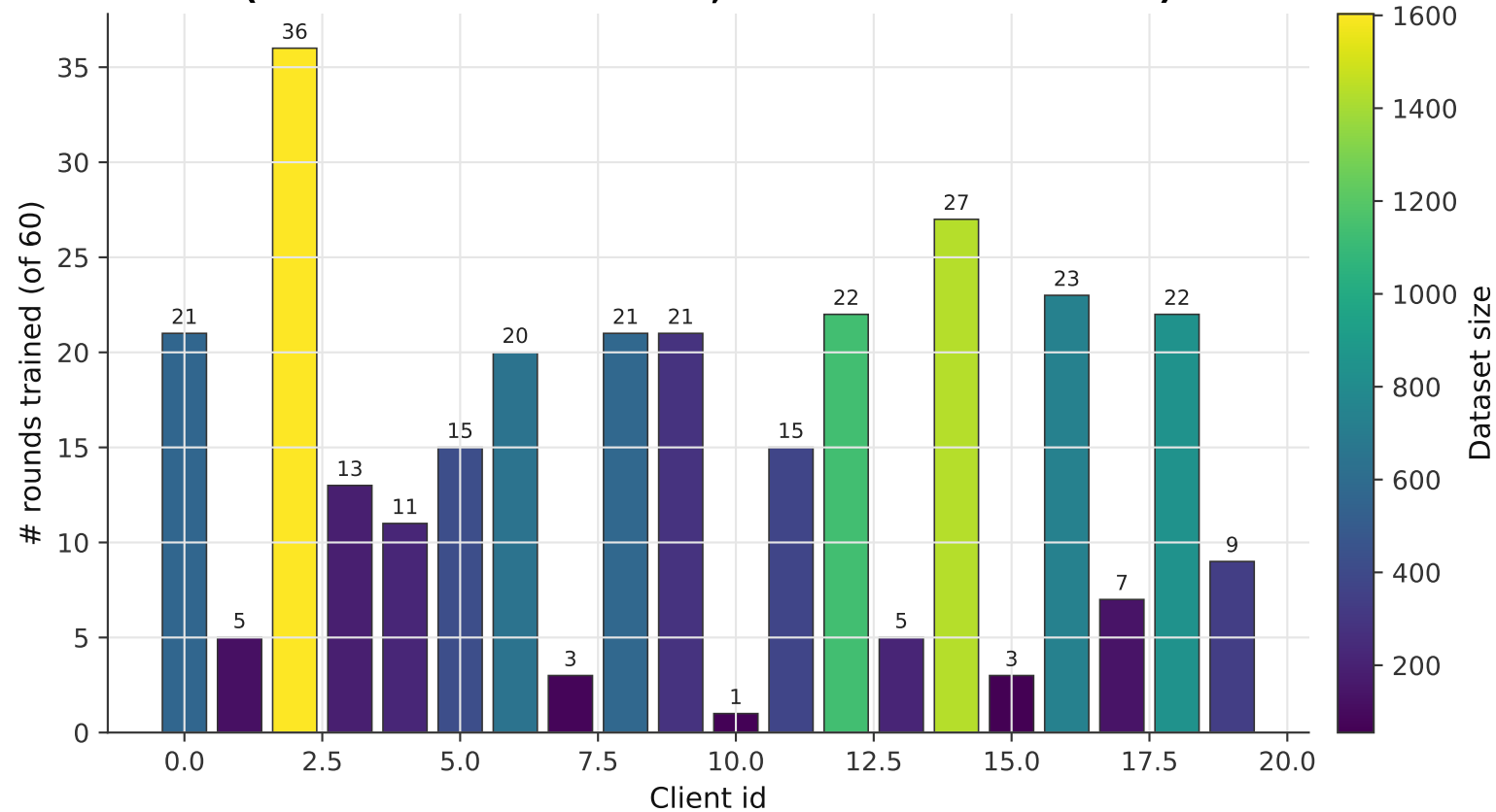
Client selection frequency — pow_d+shapfed_wa (bar color = dataset size; taller = selected more)
