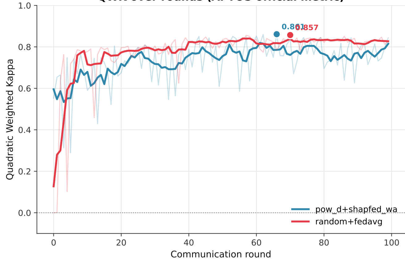
QWK over rounds (APTOS official metric)
