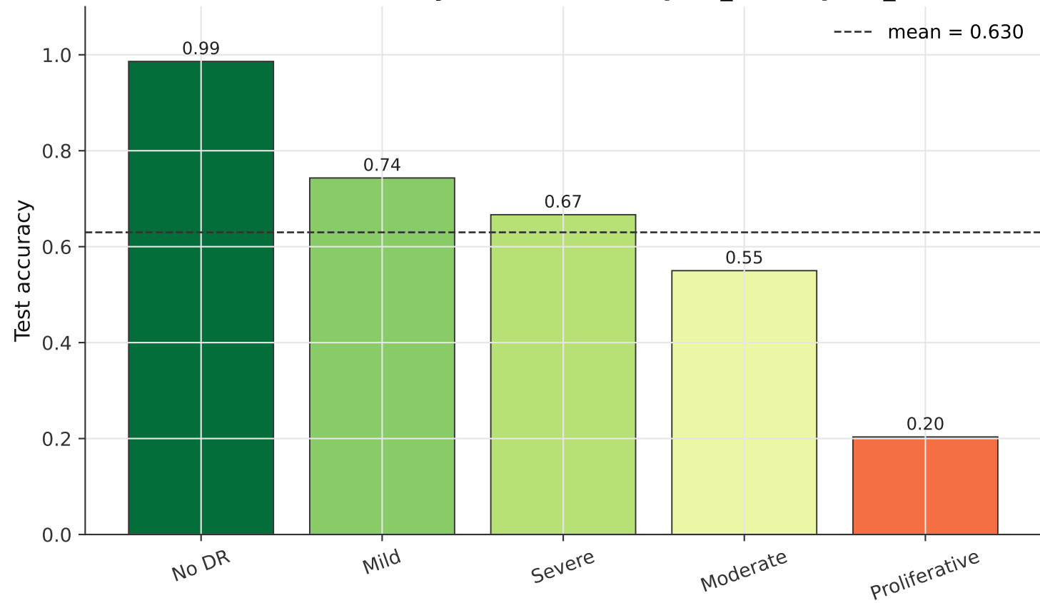
Per-class accuracy at round 99 — pow_d+shaped_wa
