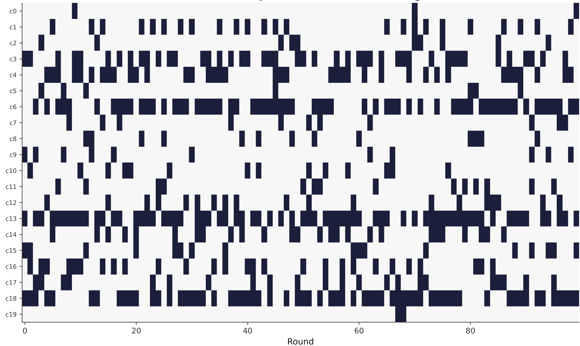
Active clients per round — random+fedavg
