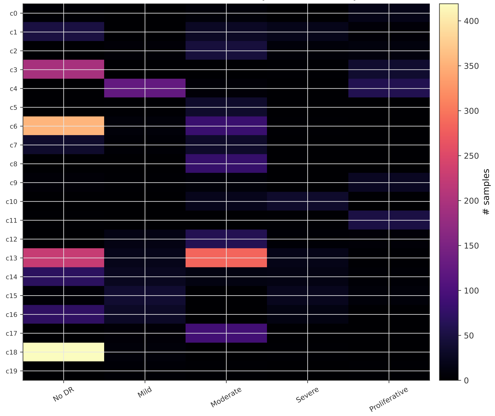
Per-client class distribution (Dirichlet \alpha=0.3 )
