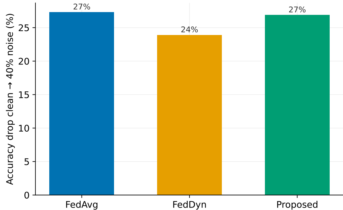
Relative accuracy lost to 40% label noise (lower = more robust)
