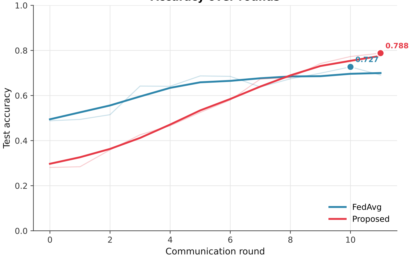
Accuracy over rounds
