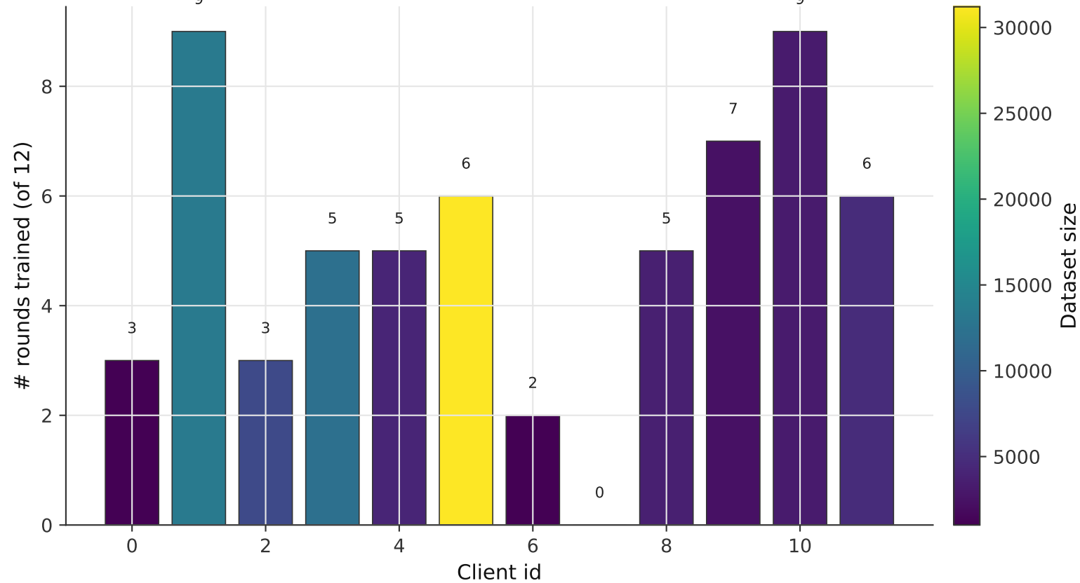
Client selection frequency — Proposed (bar color = dataset size; taller = selected more)
