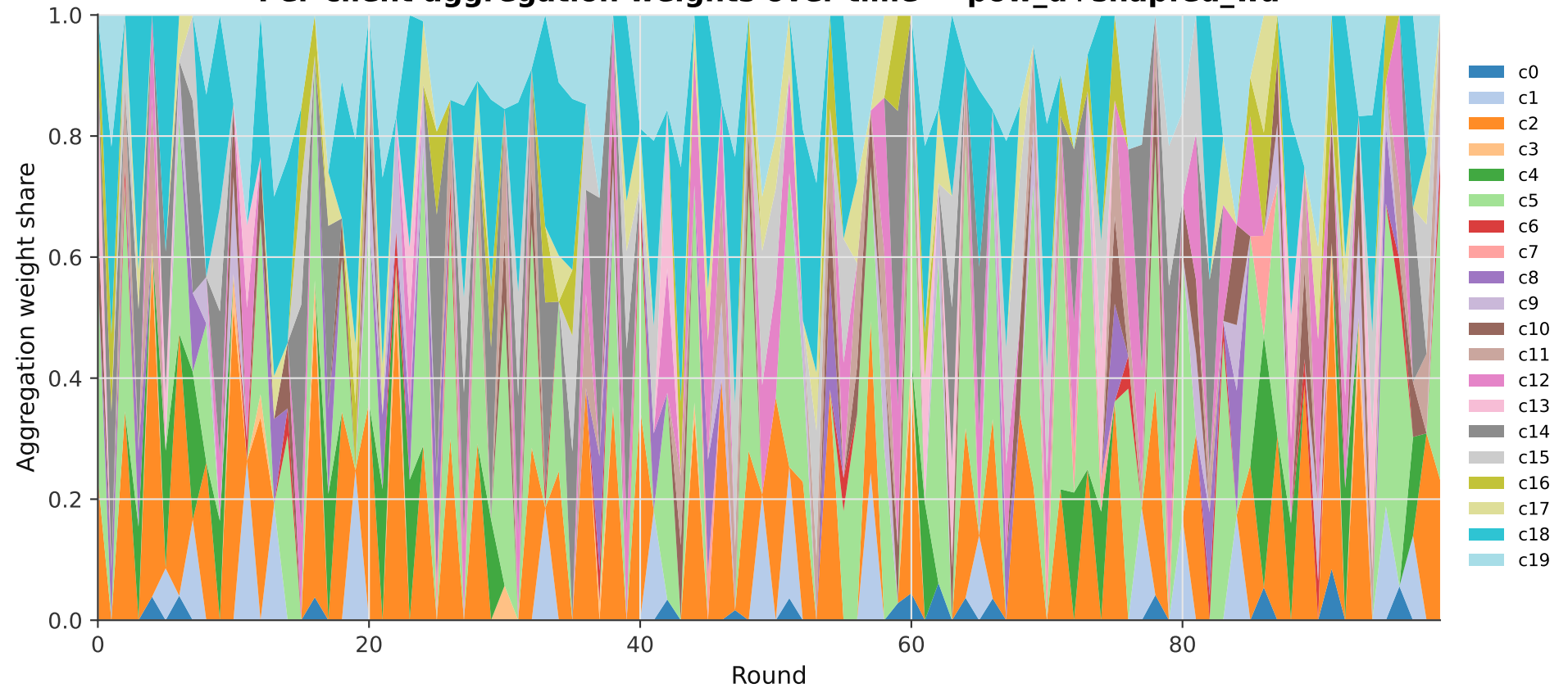
Per-client aggregation weights over time — pow_d+shapfed_wa
